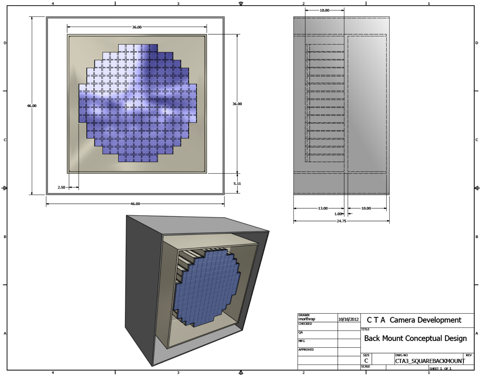
Rear Bulkhead Mount Concept
