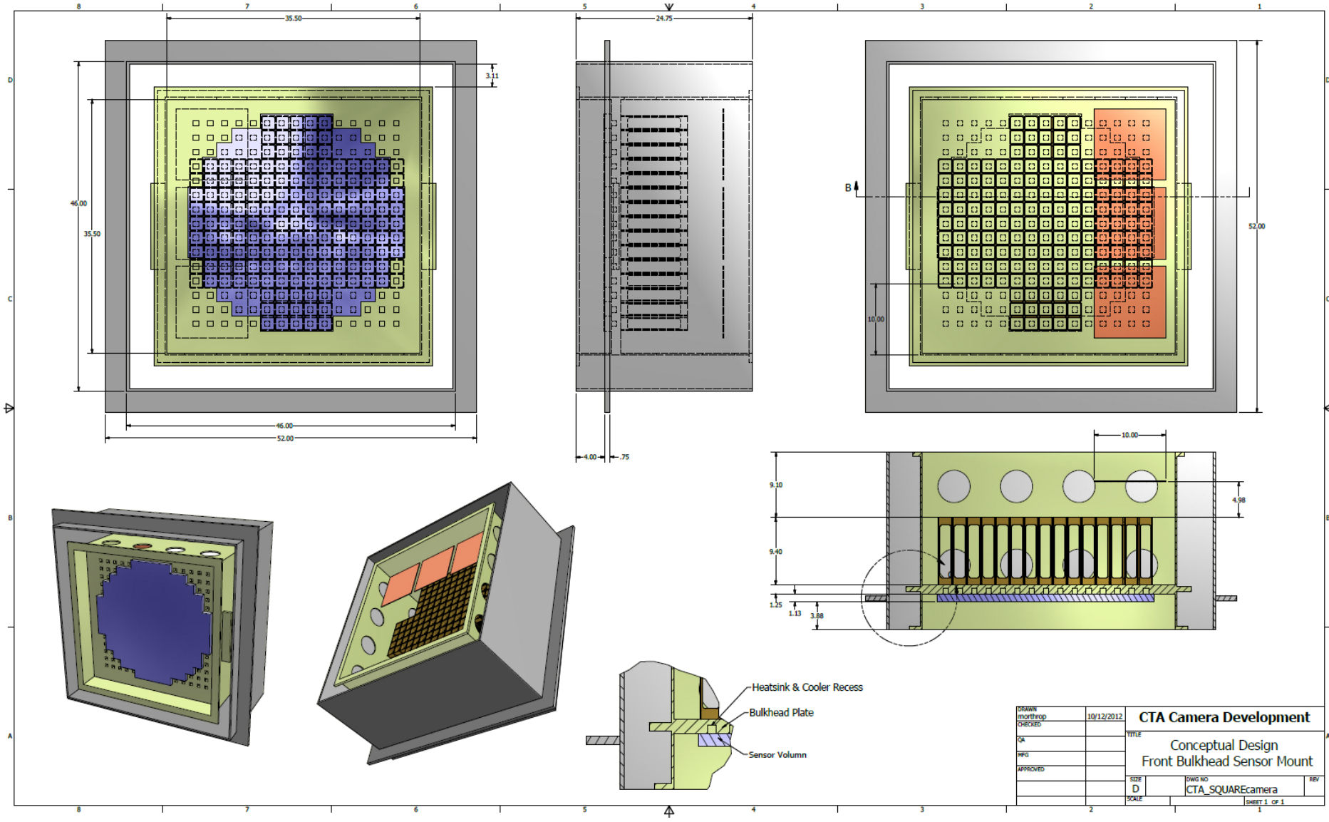
Front Bulkhead Mount Concept
