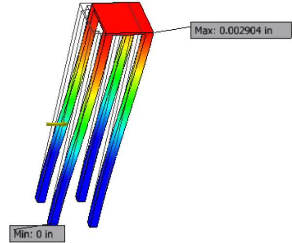
Deflections with 2 lb. UDL
