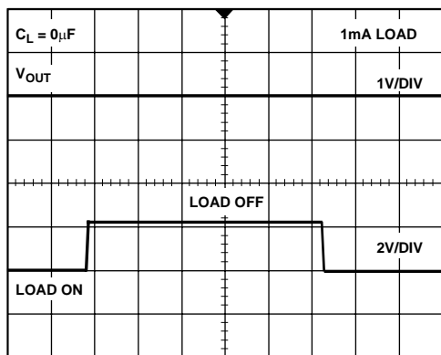
Figure 30. ADR421 Load Transient Response
