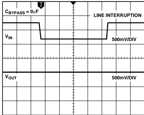
Figure 28. ADR421 Line Transient Response
