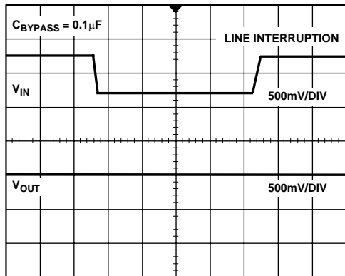
Figure 29. ADR421 Line Transient Response
