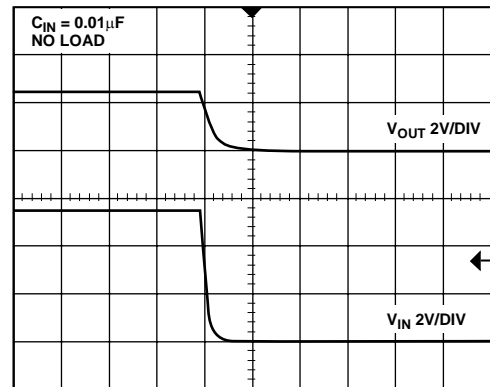
Figure 32. ADR421 Turn-Off Response
