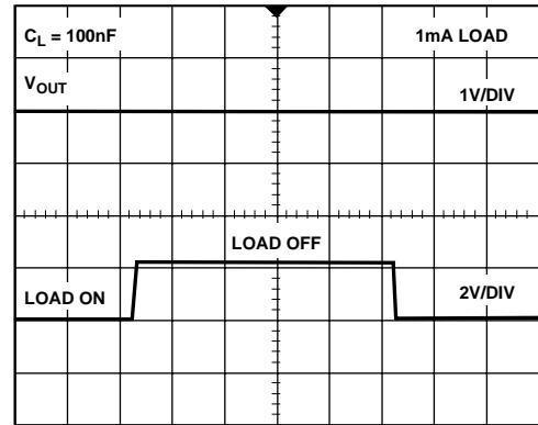
Figure 31. ADR421 Load Transient Response
