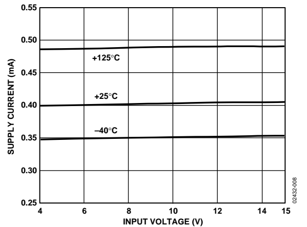
Figure 8. ADR420 Supply Current vs. Input Voltage
