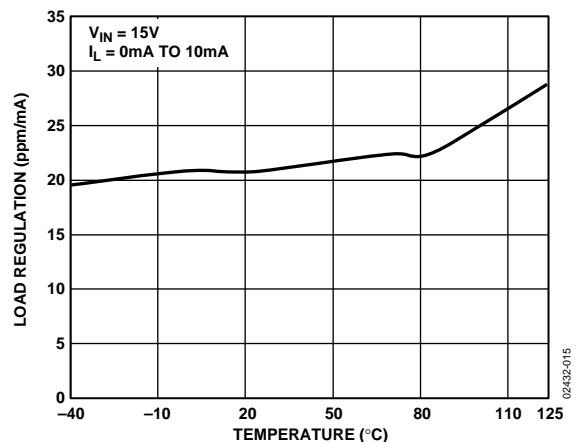
Figure 15. ADR425 Load Regulation vs. Temperature
