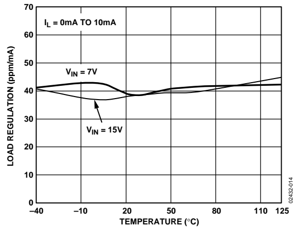
Figure 14. ADR423 Load Regulation vs. Temperature
