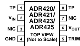
Figure 1. 8-Lead SOIC, 8-Lead MSOP
