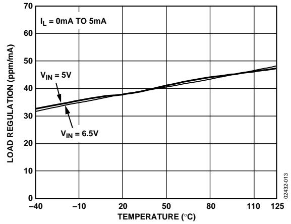
Figure 13. ADR421 Load Regulation vs. Temperature
