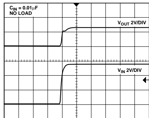
Figure 33. ADR421 Turn-On Response
