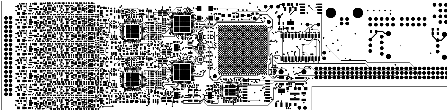
Film1 - COMPONENT SIDE SIGNAL_1
