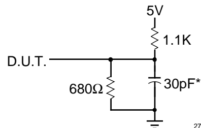
Figure 1. Output Load
