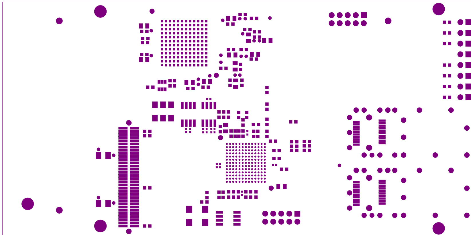
ARTWORK_11: TOP SOLDER MASK
