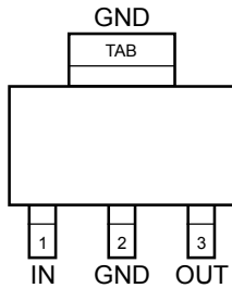
MIC37100-x.x (Fixed) SOT-223 (S)
