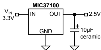
2.5V/1A Regulator
