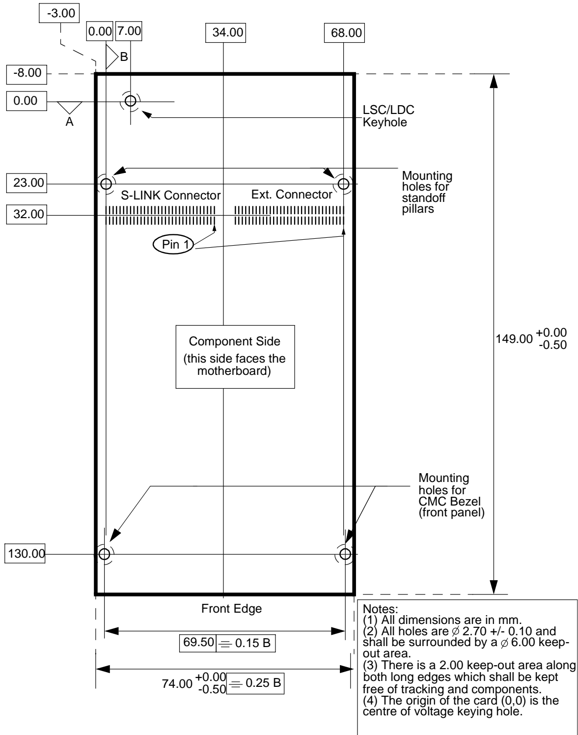
FIGURE 4. S-LINK64 card
