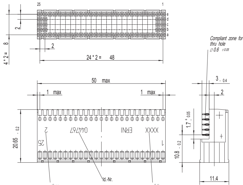
Board hole pattern (Component mounting side)
