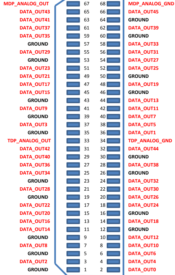
OPTOCOUPLER BOARD
