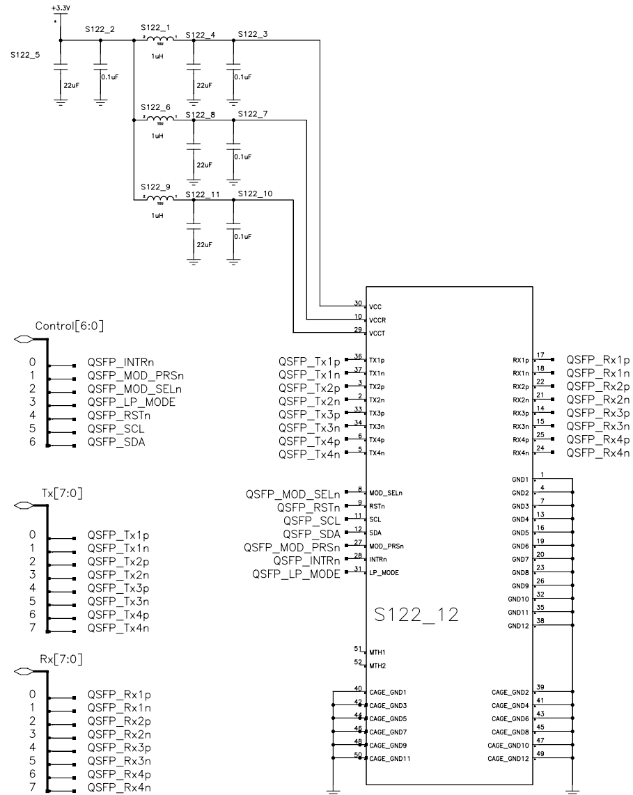
QSFP+ Module QSFP+ Cage iPASS R/A Connector, 38-pin
