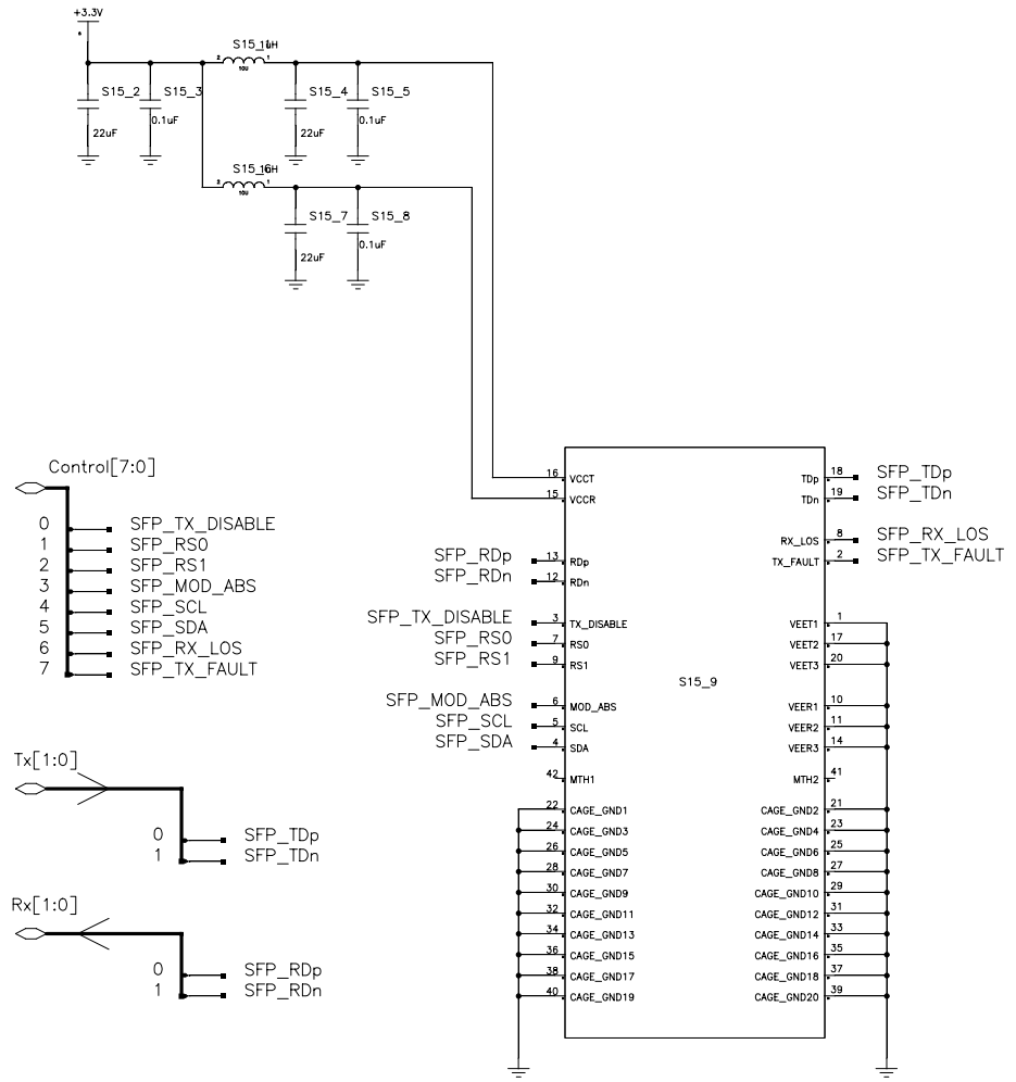
SFP+ Module SFP Cage SFP+ Host Connector, 20-pin
