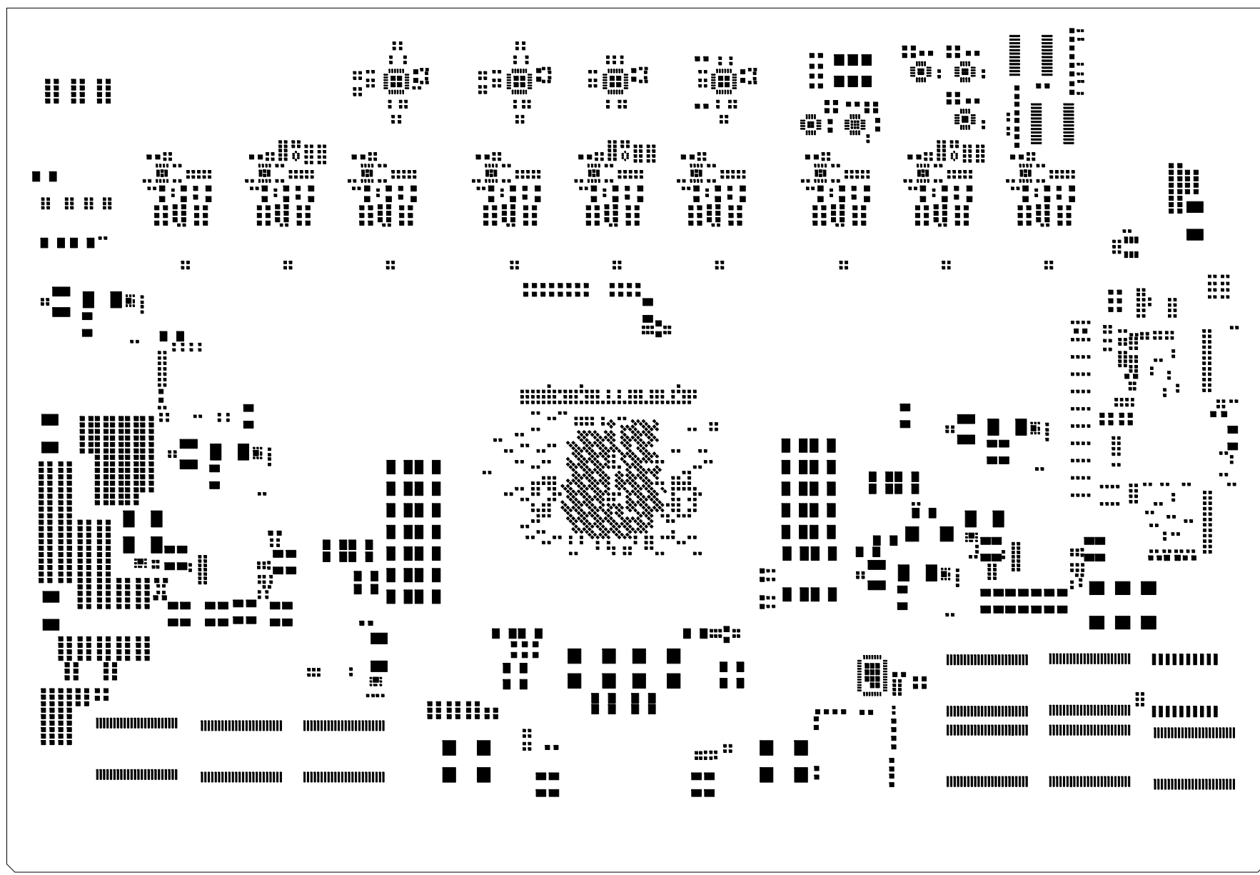
Artwork_22: Bot Pastemask
